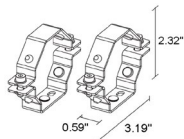
WMA05 Pair of temper-resistant clips
