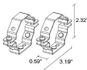
WMA05 Pair of temper-resistant clips
