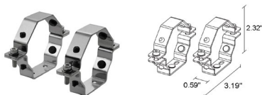
WMA05 Pair of temper-resistant clips
