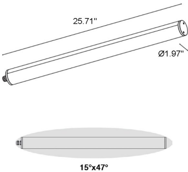
Fixture Dimensions
