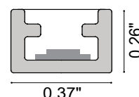
Fixture Dimensions
