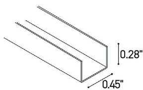
PRO-AL-9.5x6.5-AL Rigid Aluminum Outercase L=9.84'
