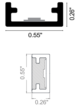
Fixture Dimensions
