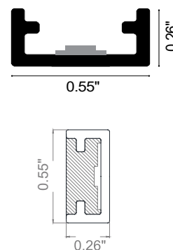
Fixture Dimensions
