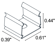
CLIP-AC-14x6.5-AC Harmonic steel clips
