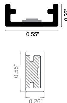
Fixture Dimensions
