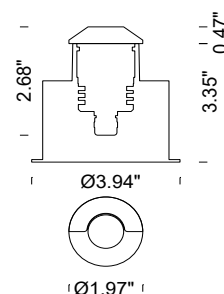
Fixture Dimensions
