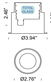
FLEA MAXI Recessed Round Trimless (Total Glass)
