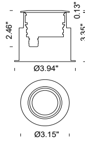
FLEA MAXI Recessed Round Trim
