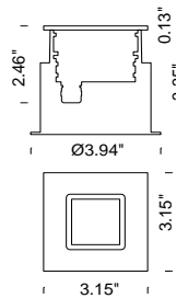
FLEA MAXI Recessed Square Trim
