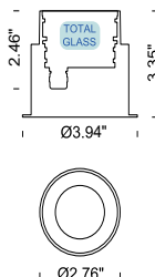
FLEA MAXI Recessed Round Trimless (Total Glass)
