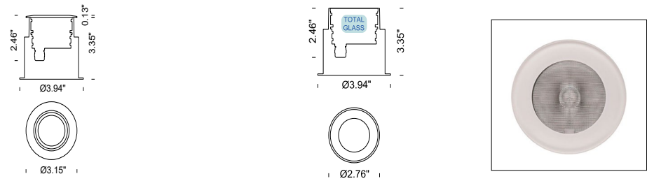
FLEA MAXI Recessed Round Trim
