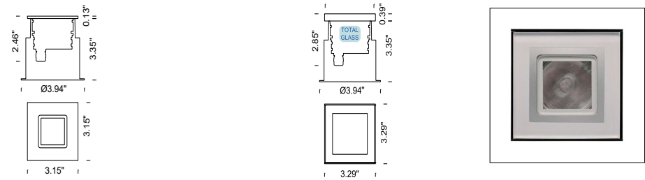
FLEA MAXI Recessed Square Trim
