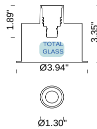
FLEA MINI Recessed Round Trimless (Total Glass)
