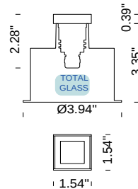
FLEA MINI Recessed Square Trimless (Total Glass)
