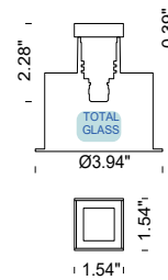
FLEA MINI Recessed Square Trimless (Total Glass)
