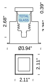
FLEA Recessed Square Trimless (Total Glass)
