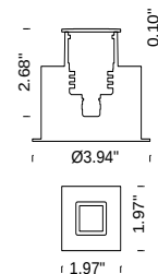
FLEA Recessed Square Trim
