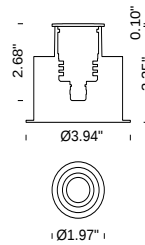
FLEA Recessed Round Trim
