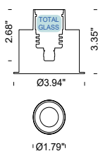
FLEA Recessed Round Trimless (Total Glass)
