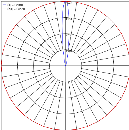
PHOTOMETRIC FILENAME : FLEA RECESSED RD 30K 10°-10133.X.3.01.IES
