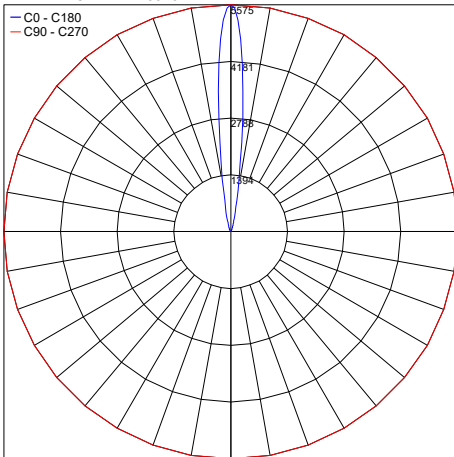
PHOTOMETRIC FILENAME : FLEA RECESSED SQ 30K 10°-10134.X.3.01.IES
