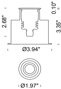
FLEA Recessed Round Trim
