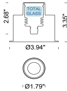
FLEA Recessed Round Trimless (Total Glass)
