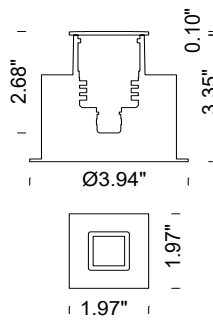
FLEA Recessed Square Trim
