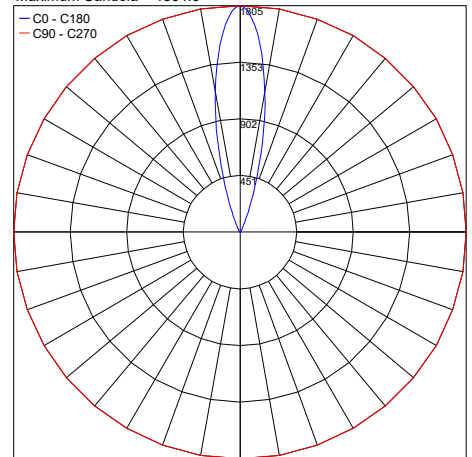
PHOTOMETRIC FILENAME : FLEA RECESSED RD 30K 30°-10133.X.3.02.IES
