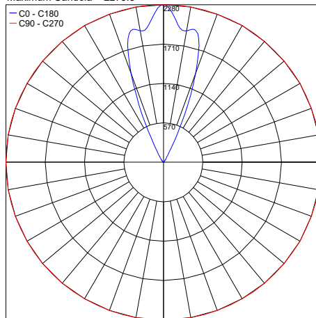
PHOTOMETRIC FILENAME : FLEA RECESSED SQ 30K 14°X20°-10134.X.3.04.IES
