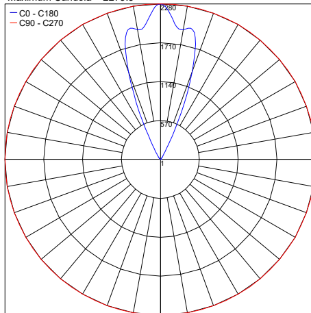
PHOTOMETRIC FILENAME : FLEA RECESSED RD 30K 14°X20°-10133.X.3.04.IES
