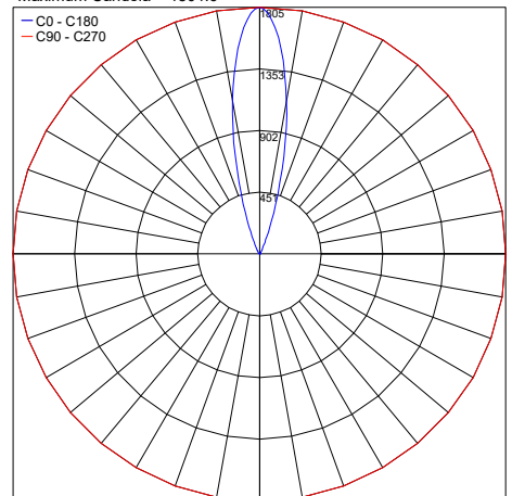
PHOTOMETRIC FILENAME : FLEA RECESSED SQ 30K 30°-10134.X.3.02.IES
