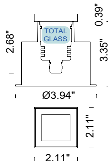
FLEA Recessed Square Trimless (Total Glass)
