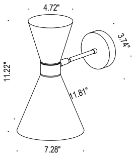
Fixture Dimensions
