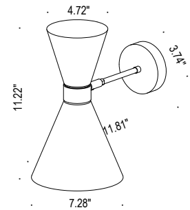
Fixture Dimensions
