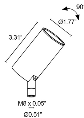
Fixture Dimensions
