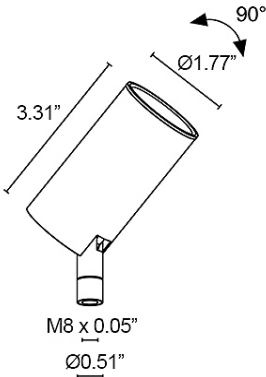
Fixture Dimensions
