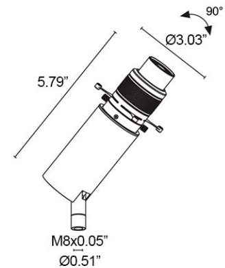
Fixture Dimensions
