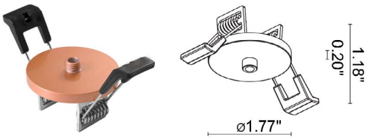
WGA09B - White WGA09N - Black WGA09Y - Rose Gold WGA098Z - Antique Bronze Retaining Spring Clip \varnothing 1.77 "
