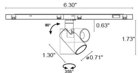
Fixture Dimensions
