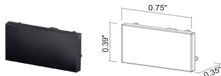
BE0031000 End Cap - Surface-mounted track
