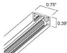
BE0030025 Surface-mounted Track 6.56' (2 m)
