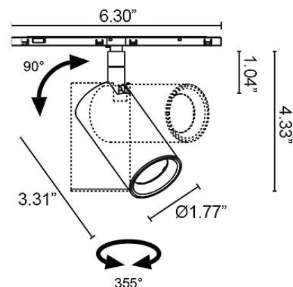
Fixture Dimensions
