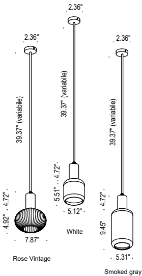
Fixture Dimensions
