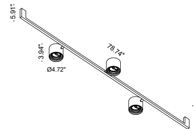
Fixture Dimensions
