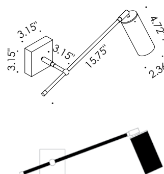
Fixture Dimensions
