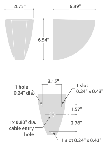
Fixture Dimensions
