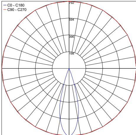
PHOTOMETRIC FILENAME : ELITE_C_3000K_MEDIUM_BEAM_CC_HO_1.5IN.IES
