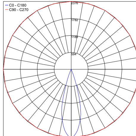
PHOTOMETRIC FILENAME : ELITE_C_3000K_MEDIUM_BEAM_CC_HO_4.0IN.IES
