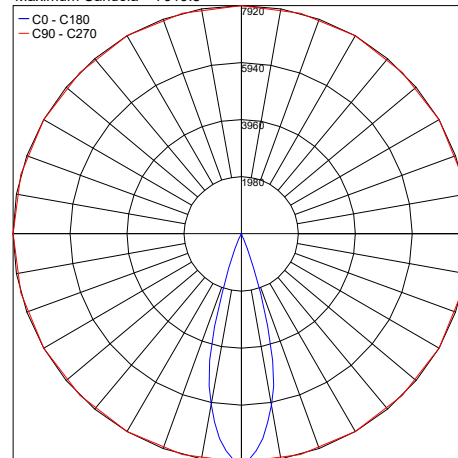
PHOTOMETRIC FILENAME : ELITE_C_3000K_MEDIUM_BEAM_CC_HO_12.9IN.IES
