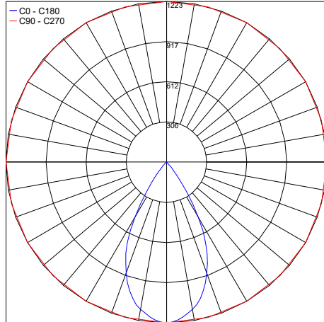
PHOTOMETRIC FILENAME : ELITE_C_3000K_WIDE_BEAM_CC_HO_6.6IN.IES
