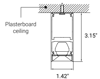
Fixture Dimensions
