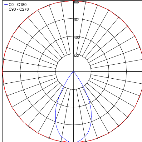
PHOTOMETRIC FILENAME : ELITE_C_3000K_WIDE_BEAM_CC_HO_2.8IN.IES
