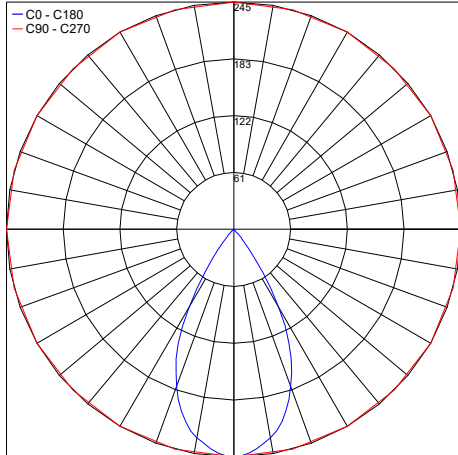
PHOTOMETRIC FILENAME : ELITE_C_3000K_WIDE_BEAM_CC_HO_1.5IN.IES
