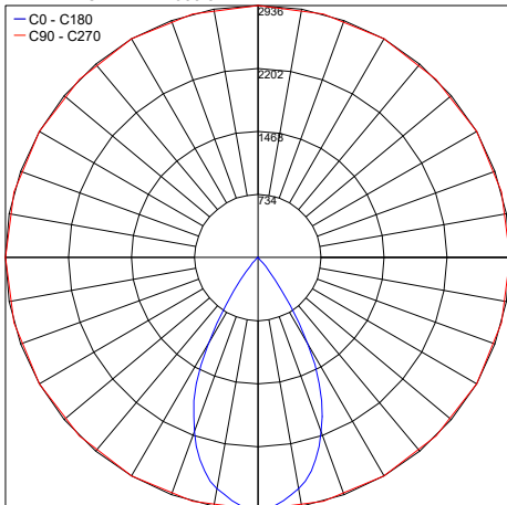
PHOTOMETRIC FILENAME : ELITE_C_3000K_WIDE_BEAM_CC_HO_15.4IN.IES
