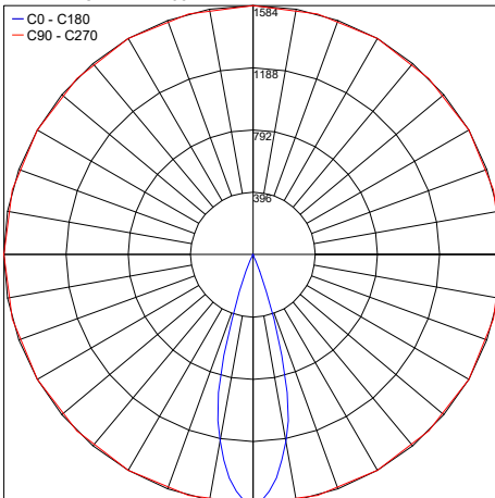
PHOTOMETRIC FILENAME : ELITE_C_3000K_MEDIUM_BEAM_CC_HO_2.8IN.IES
