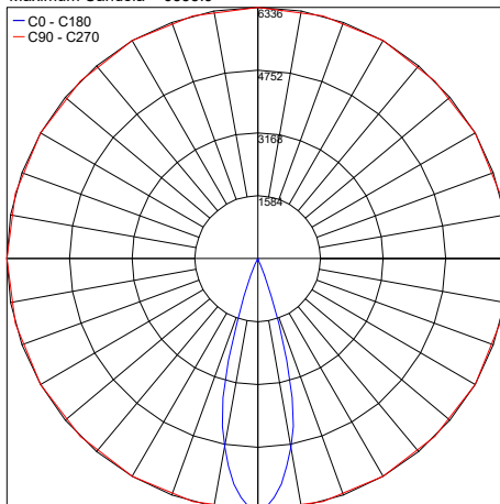
PHOTOMETRIC FILENAME : ELITE_C_3000K_MEDIUM_BEAM_CC_HO_10.4IN.IES
