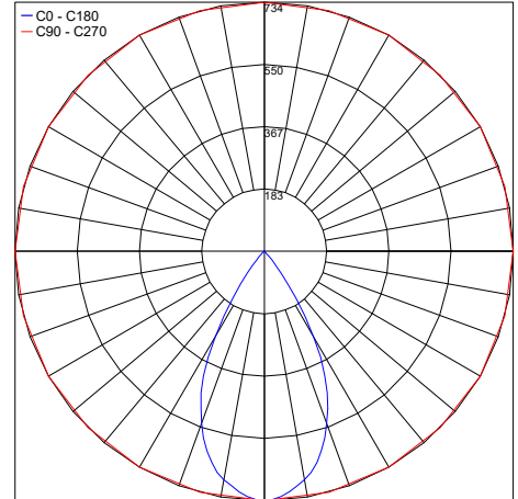
PHOTOMETRIC FILENAME : ELITE_C_3000K_WIDE_BEAM_CC_HO_4.0IN.IES
