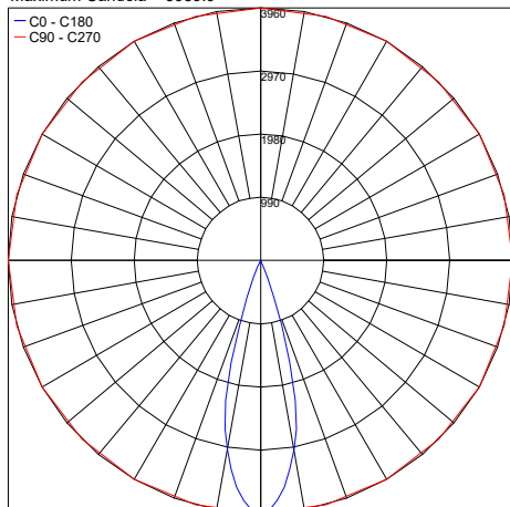
PHOTOMETRIC FILENAME : ELITE_C_3000K_MEDIUM_BEAM_CC_HO_6.6IN.IES
