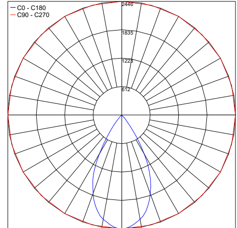
PHOTOMETRIC FILENAME : ELITE_C_3000K_WIDE_BEAM_CC_HO_12.9IN.IES
