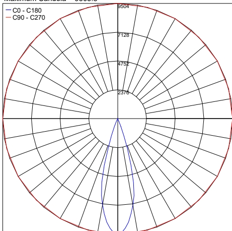
PHOTOMETRIC FILENAME : ELITE_C_3000K_MEDIUM_BEAM_CC_HO_15.4IN.IES
