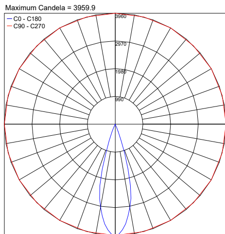
PHOTOMETRIC FILENAME : ELITE_F_3000K_MEDIUM_30°_CC_HO_7.1IN.IES
