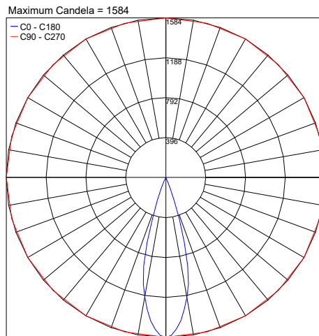
PHOTOMETRIC FILENAME : ELITE_F_3000K_MEDIUM_30°_CC_HO_3.3IN.IES
