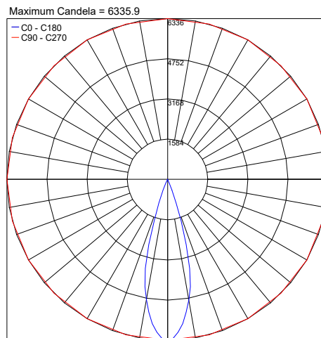
PHOTOMETRIC FILENAME : ELITE_F_3000K_MEDIUM_30°_CC_HO_10.9IN.IES
