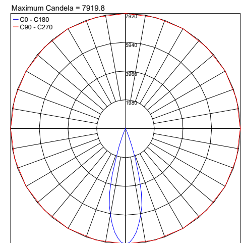
PHOTOMETRIC FILENAME : ELITE_F_3000K_MEDIUM_30°_CC_HO_13.4IN.IES
