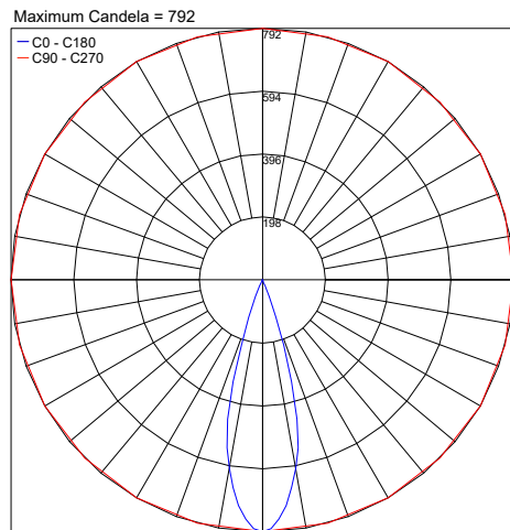
PHOTOMETRIC FILENAME : ELITE_F_3000K_MEDIUM_30°_CC_HO_2.1IN.IES
