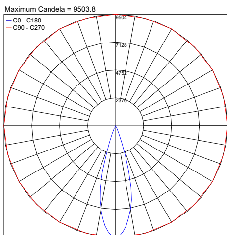
PHOTOMETRIC FILENAME : ELITE_F_3000K_MEDIUM_30°_CC_HO_15.9IN.IES
