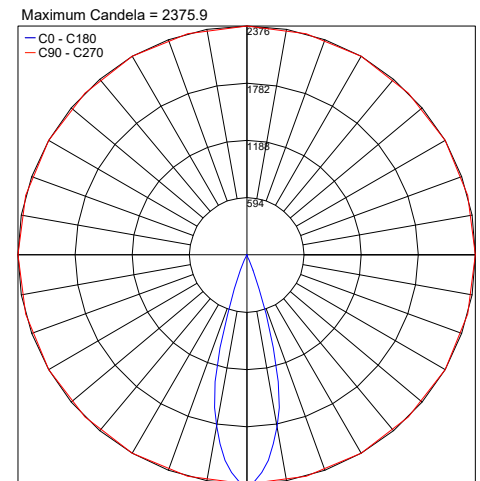
PHOTOMETRIC FILENAME : ELITE_F_3000K_MEDIUM_30°_CC_HO_4.6IN.IES
