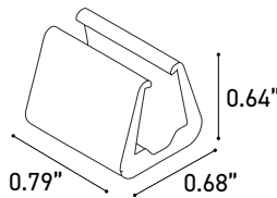
CLIP-S-8x9.5.F/W Silicone Clip
