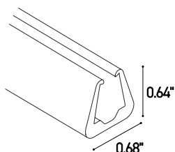
OUT-S-10x11.F/W Flexible Silicone Outercase Max L=32.81'
