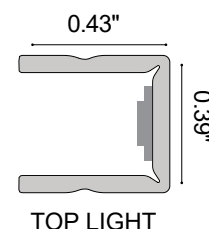
Fixture Dimensions
