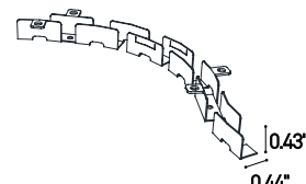
SNK2-AC-10x11-AC Flexible Steel Profile for Plasterboard L = 3.28'
