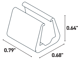
CLIP-S-10x11.F/W Sylicone clips to press-in the LED Strip
