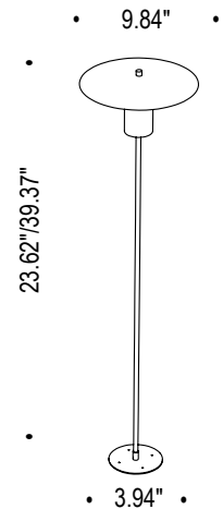
Fixture Dimensions
