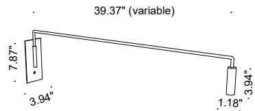
Fixture Dimensions
