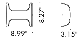
Fixture Dimensions
