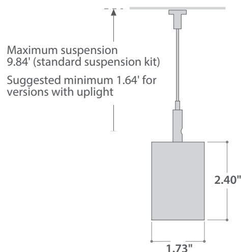
Suspended Version
