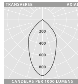
BROAD DISTRIBUTION BLACK OUTER REFLECTOR
