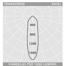
NARROW DISTRIBUTION WHITE OUTER REFLECTOR
