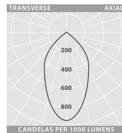
BROAD DISTRIBUTION WHITE OUTER REFLECTOR
