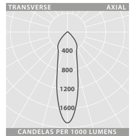
NARROW DISTRIBUTION BLACK OUTER REFLECTOR
