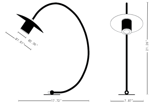
Fixture Dimensions
