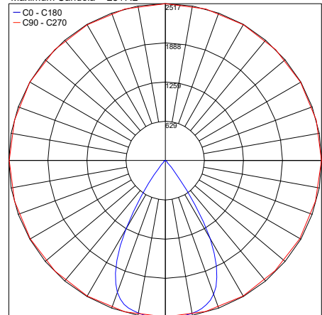
PANEL 12 C RECTANGLE Medium Output
