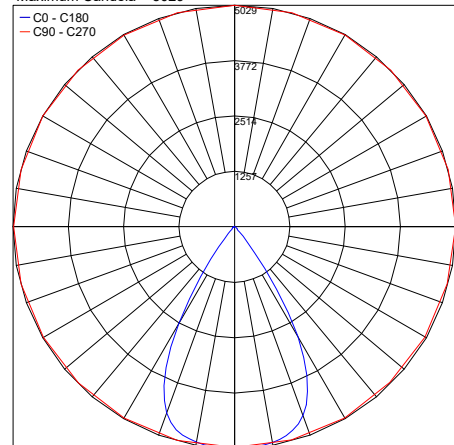
PANEL 24 C RECTANGLE Medium Output
