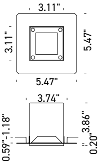
Fixture Dimensions
