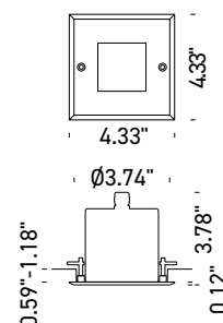
Fixture Dimensions
