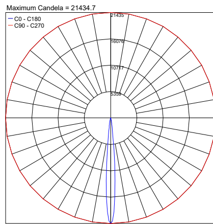
PHOTOMETRIC FILENAME : KOS DOWNLIGHT TRIM 30K 10° - 20526.X.3.01.IES
