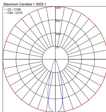
PHOTOMETRIC FILENAME : KOS DOWNLIGHT TRIM 30K 25° - 20526.X.3.36.IES
