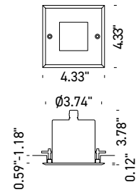
Fixture Dimensions
