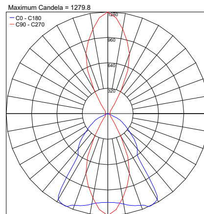
PHOTOMETRIC FILENAME : KOS DOWNLIGHT TRIM 30K 115°X20° - 20526.X.3.37.IES
