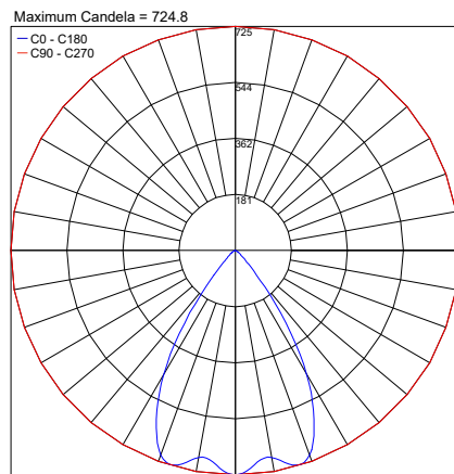
PHOTOMETRIC FILENAME : KOS DOWNLIGHT TRIM 30K 65° - 20526.X.3.34.IES
