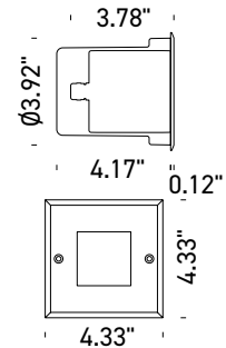
Fixture Dimensions
