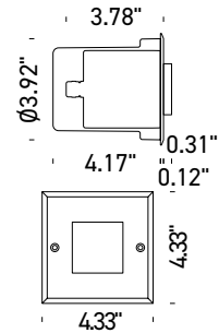
Fixture Dimensions
